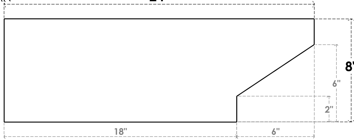
SIDE PROFILE
